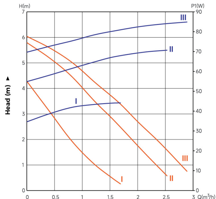
Capacity Q ► LRP15-60/130 LRP15-60B/130 — Q-P — Q-H
