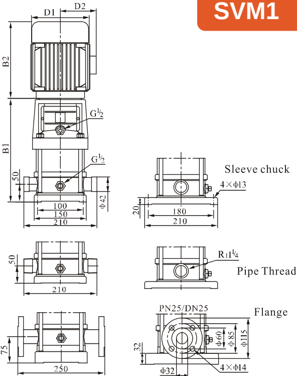
Installation drawing
