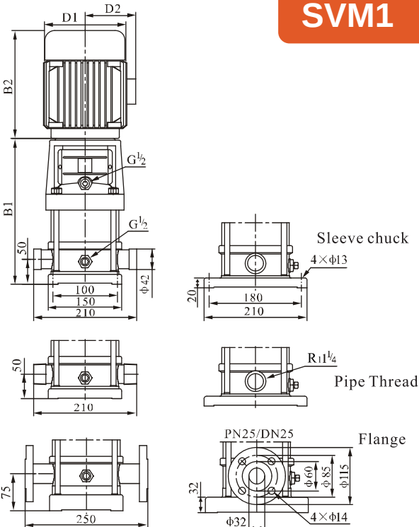
Installation drawing
