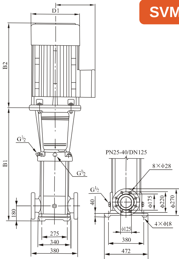
Installation drawing
