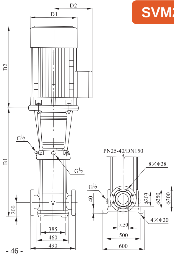
Installation drawing
