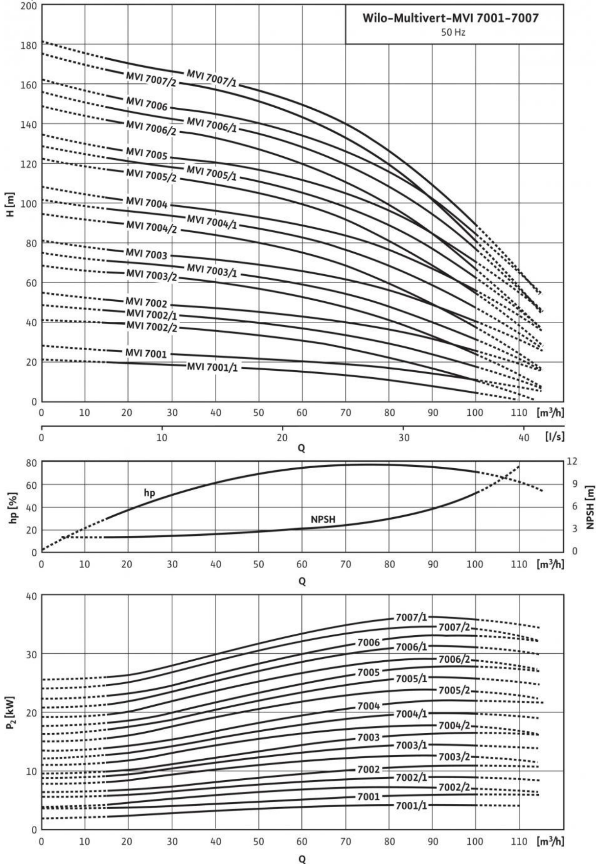
Pump curves
