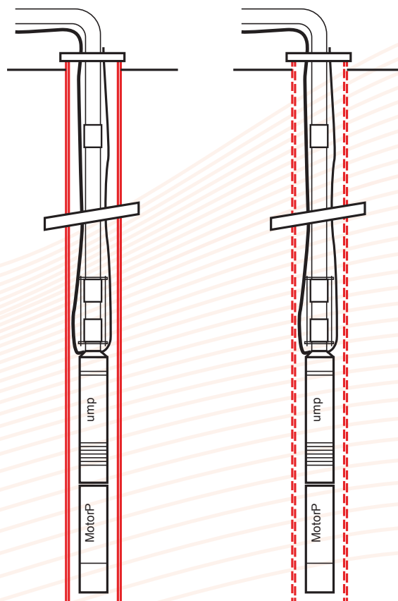
Solid vs Perforated borehole casings
