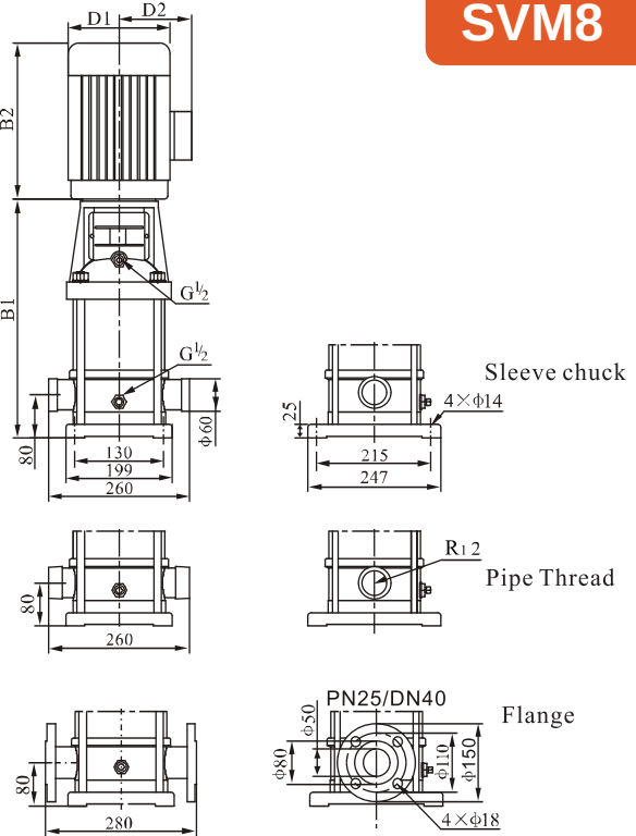
Installation drawing
