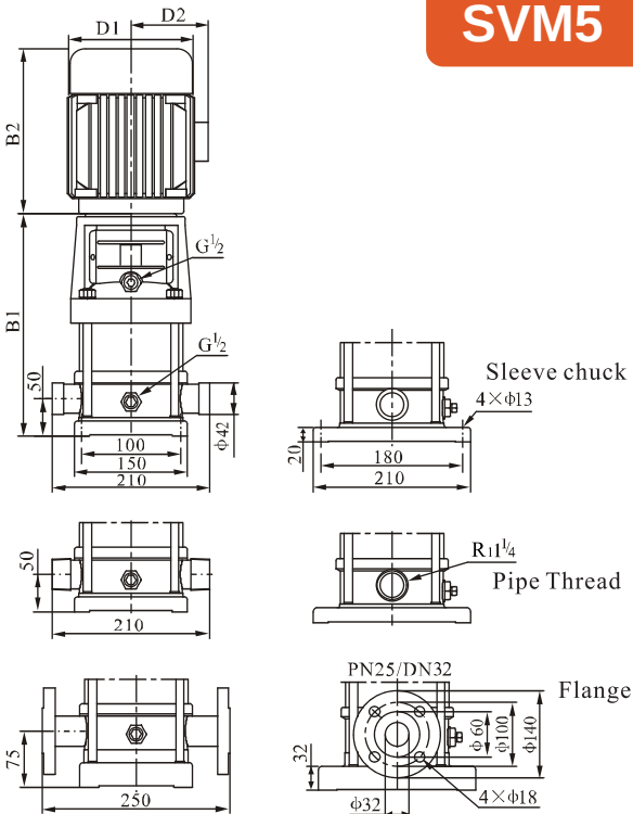
Installation drawing
